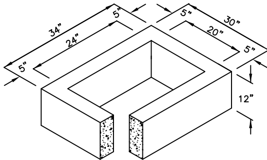
12" RISER SECTION
