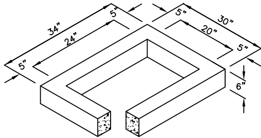
6" RISER SECTION
