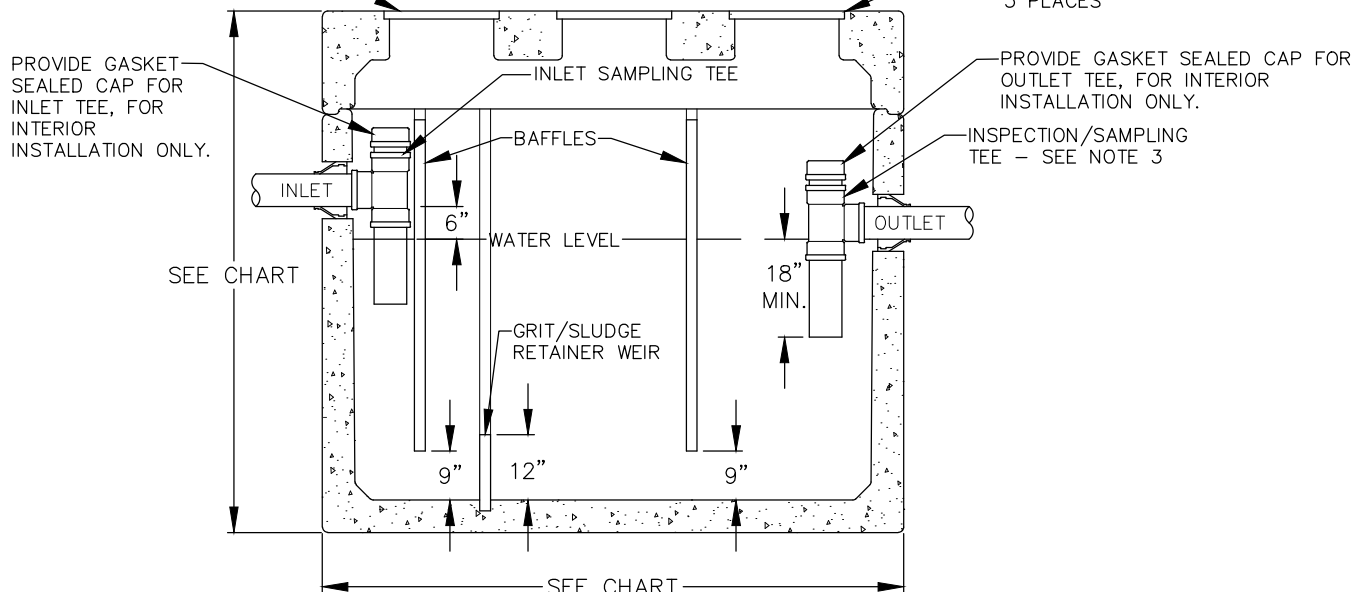
SECTION AA
